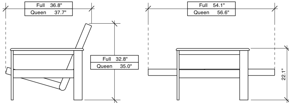
SEATING POSITION
